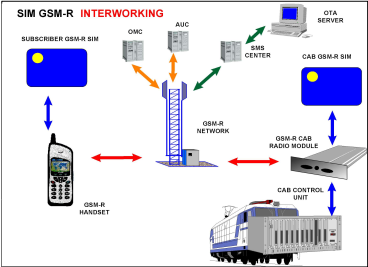
Figure 1: SIM GSM-R interworking
