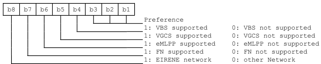
Figure 11: Structure of Class_of_network
