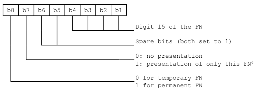
Figure 6: Structure of last byte of Functional Number and type
