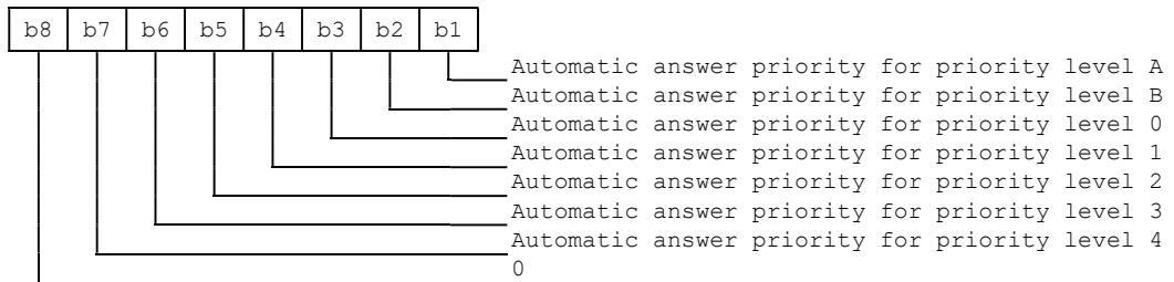
Figure 5: Byte 1 of EF AAeM
