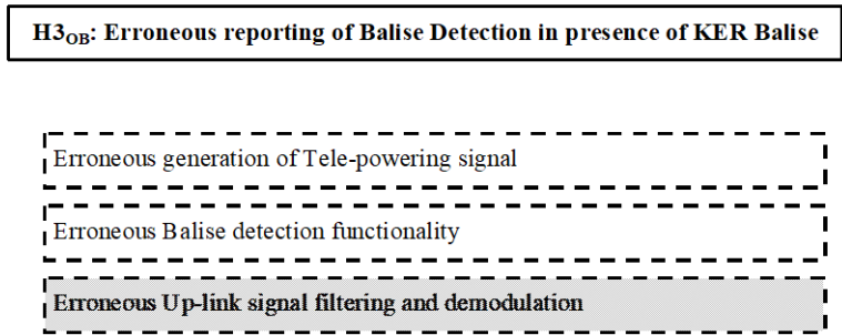
Figure 44: Erroneous Reporting of Balise Detection in presence of KER Balise
