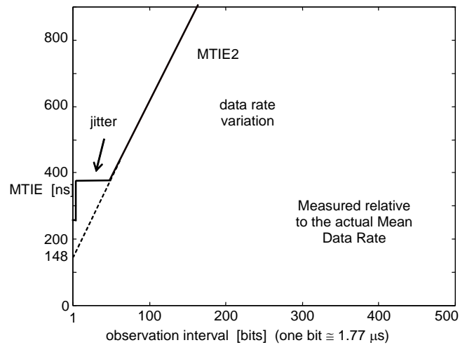
Figure 10: MTIE requirement 2
