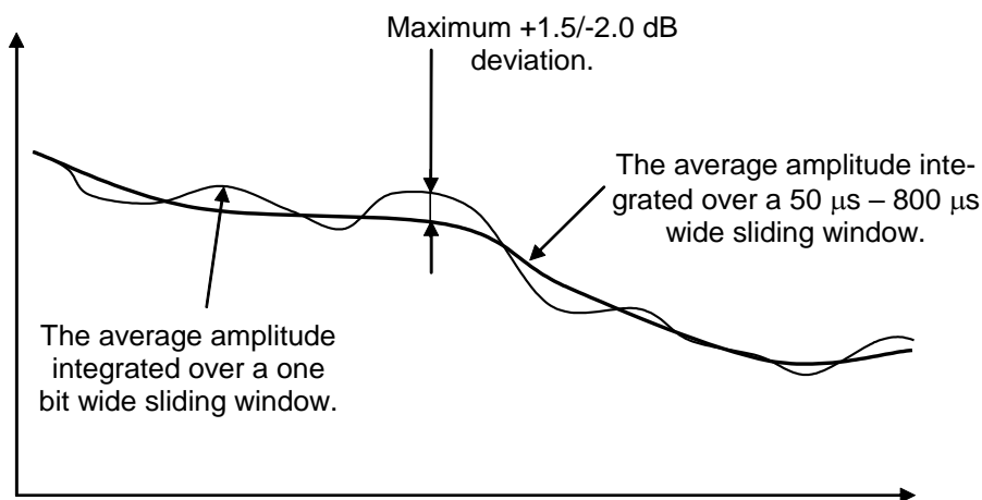
Figure 11: Amplitude jitter
