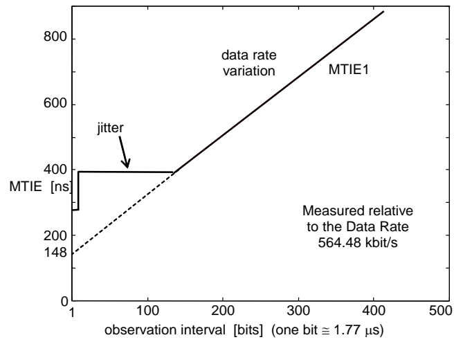
Figure 9: MTIE requirement 1
