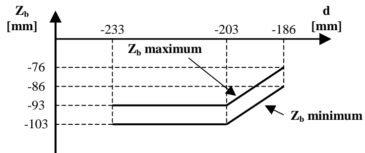
Figure 37: Mounting height, Standard Size Balise
