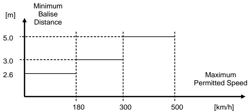
Figure 28: Minimum Distance Between Standard Size Eurobalises
