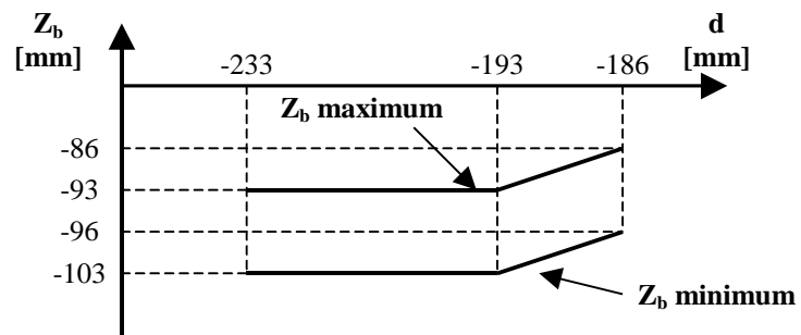
Figure 38: Mounting height, Reduced Size Balise
