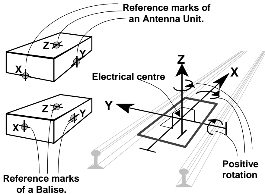
Figure 7: Reference Axes
