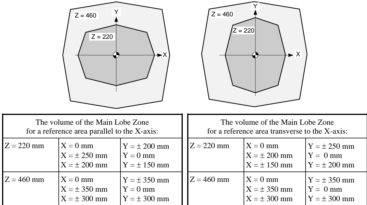
Figure 13: The volume of the Main Lobe Zone
