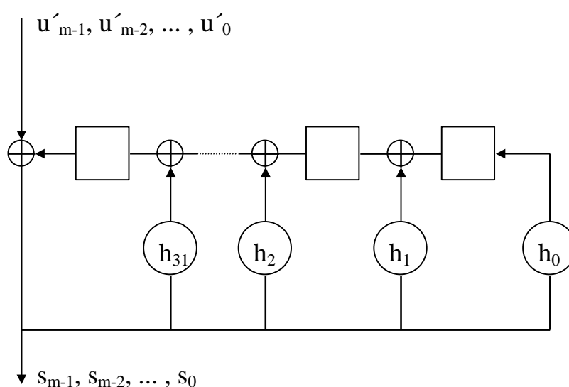
Figure 5: Scrambling
