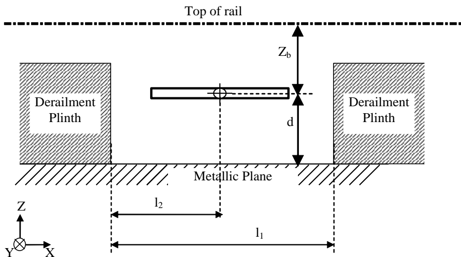
Figure 34: Derailment Plinth
