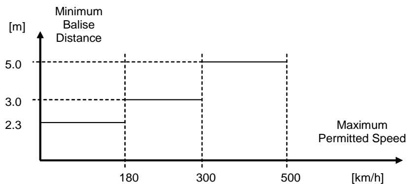
Figure 27: Minimum Distance Between Reduced Size Eurobalises
