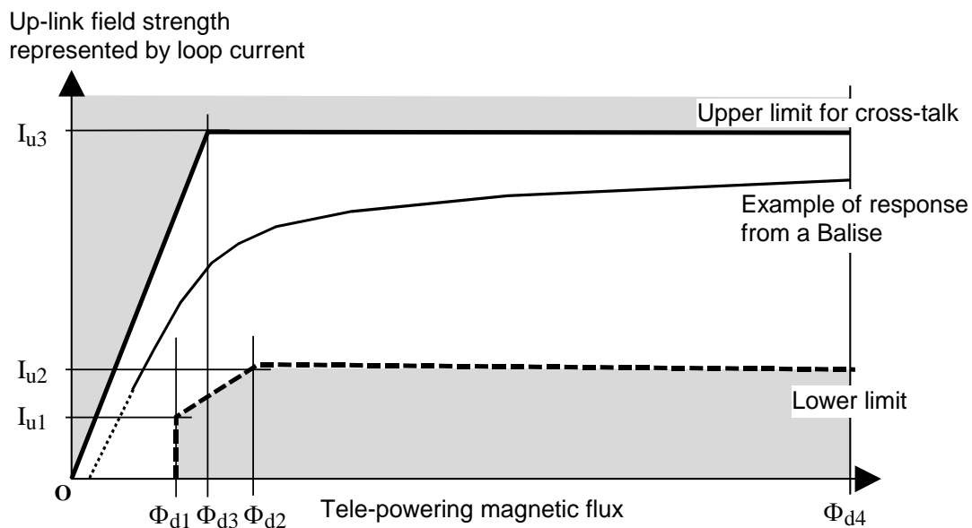
Figure 16: Input-to-output characteristics for a Balise
