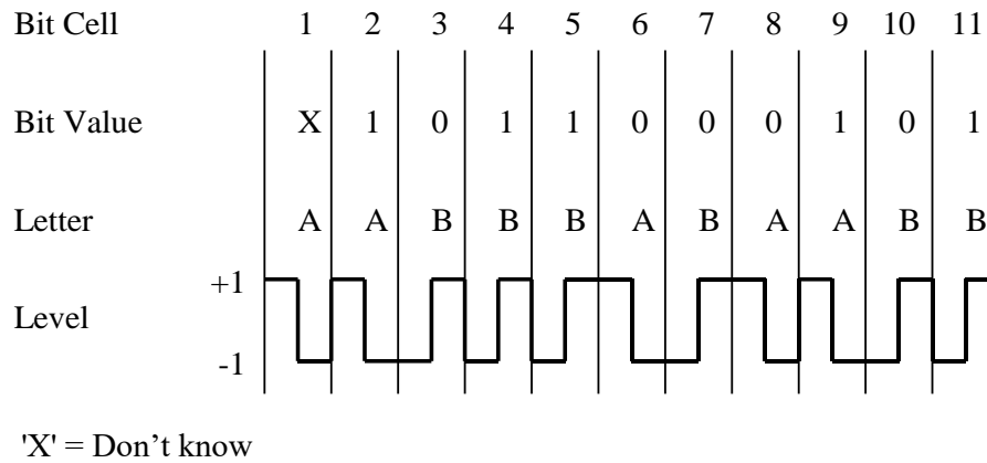
Figure 18: Differential Bi-Phase-Level coding scheme
