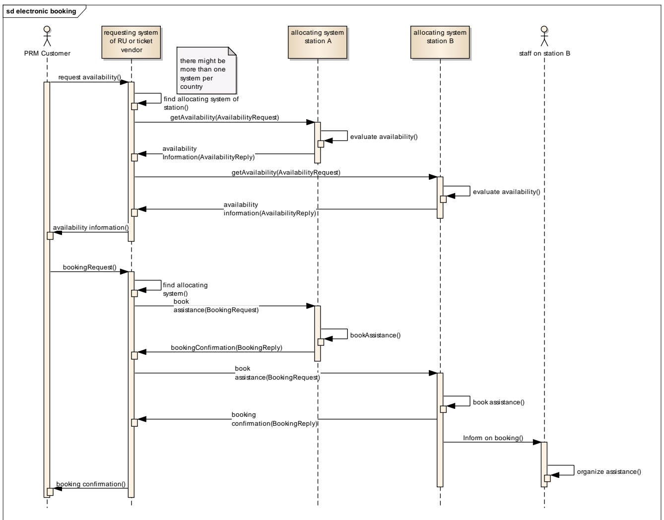
Figure 5 sequence diagram - availability and booking
