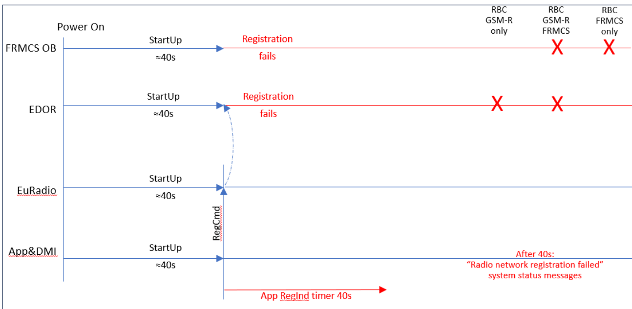
Figure 3 No GSM-R / No FRMCS available
