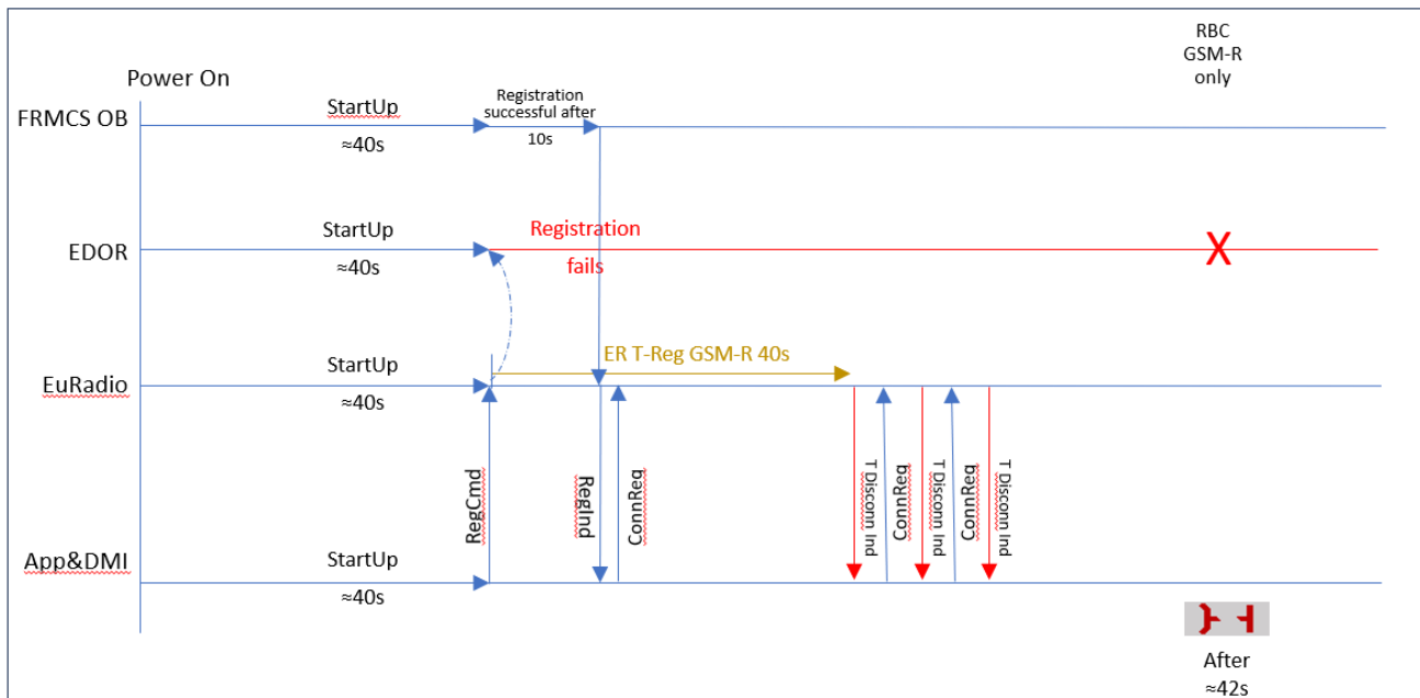
Figure 6 No GSM-R, FRMCS available, GSM-R only RBC
