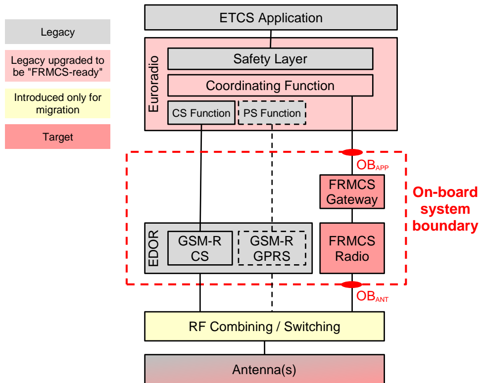
Figure 2 On-board logical architecture
