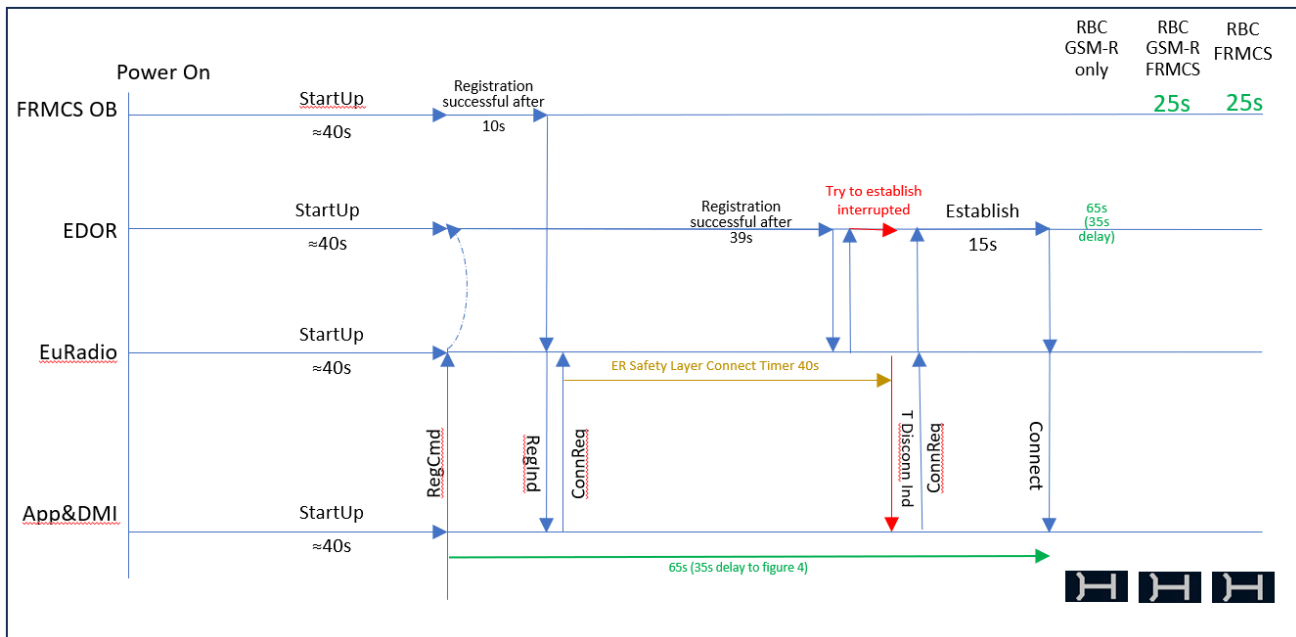
Figure 5 GSM-R / FRMCS available, but GSM-R registration late
