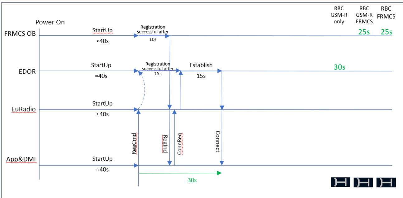
Figure 4 GSM-R / FRMCS available; normal scenario
