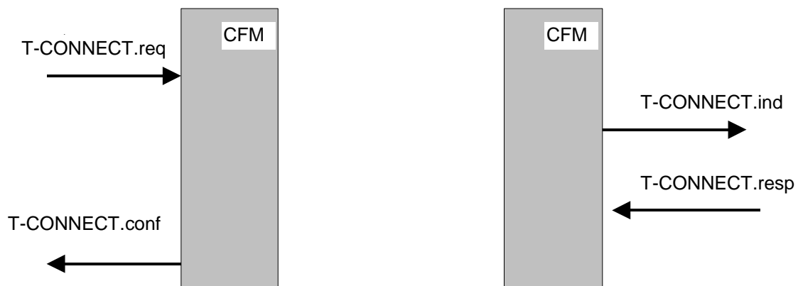
Figure 28 Sequence of primitives for connection set up
