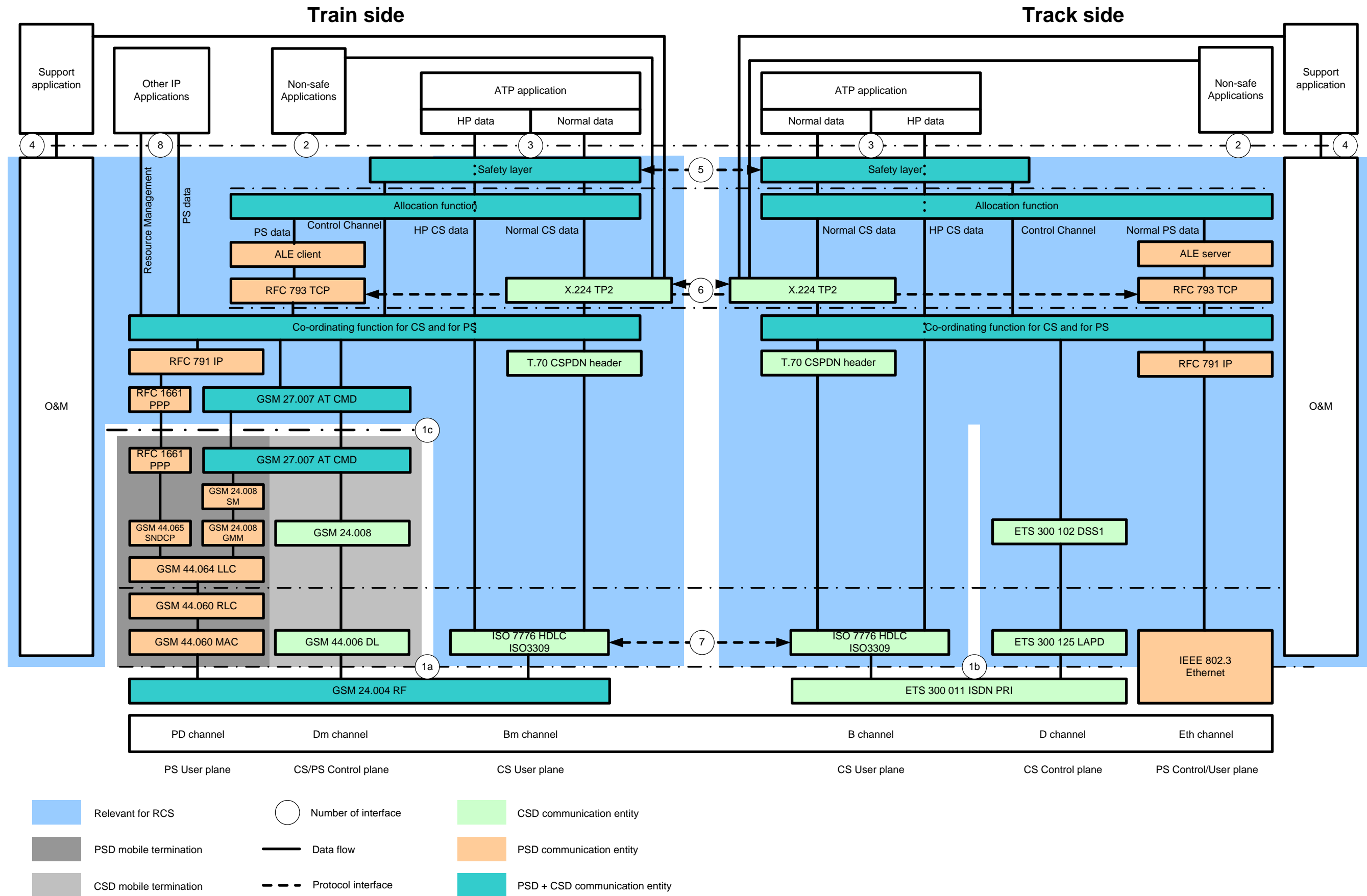
Figure 2 Reference architecture of EuroRadio system
