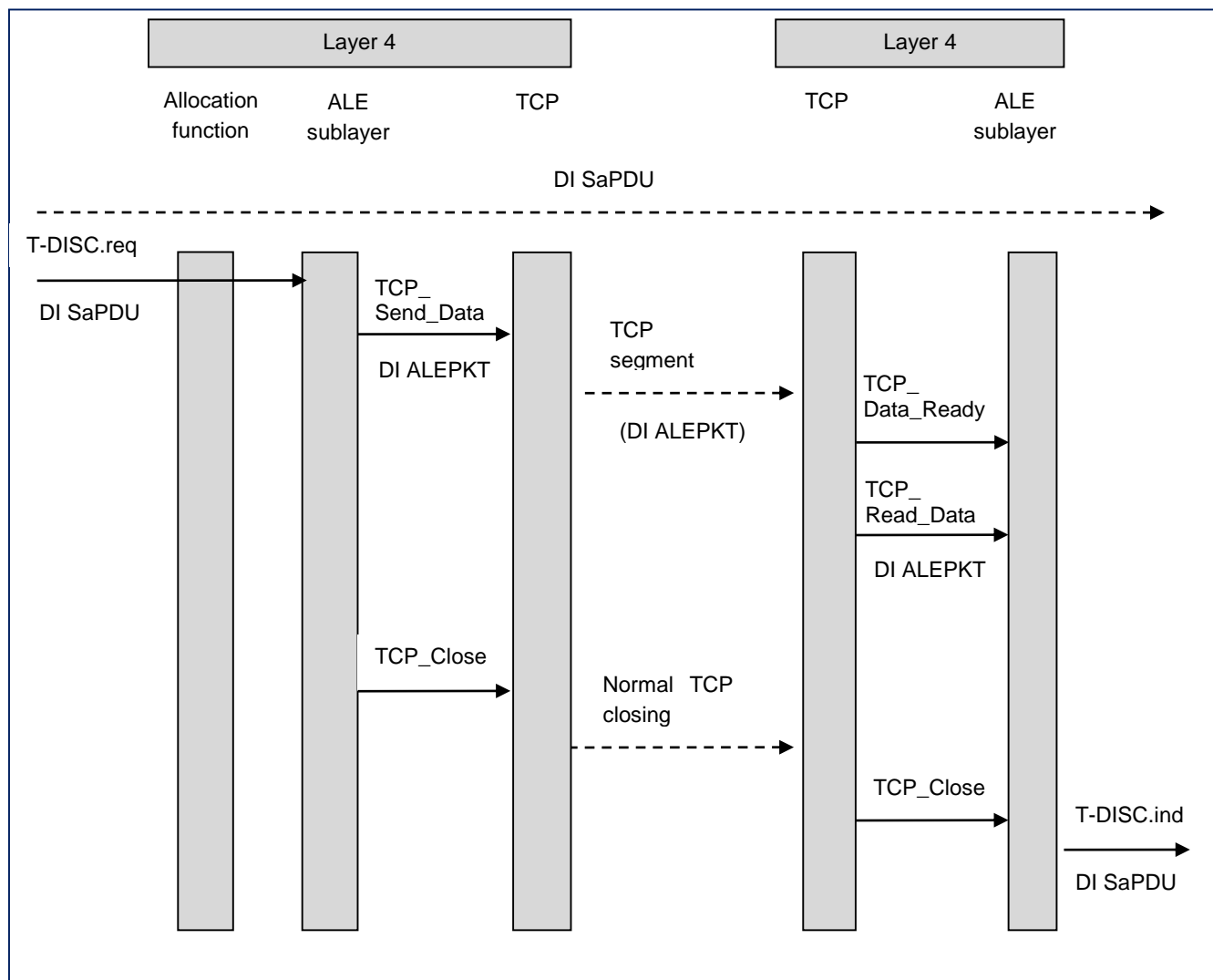
Figure 25 Time sequence "Connection Release"
