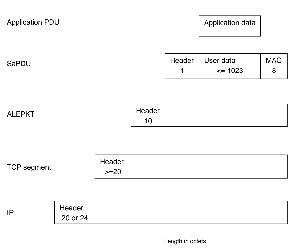
Figure 26 Relation between PDUs
