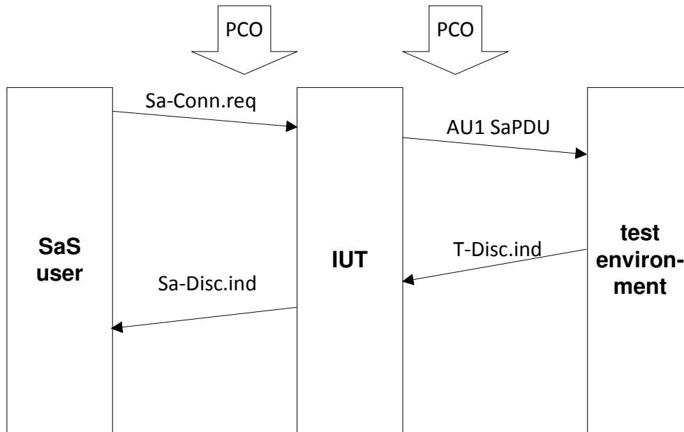
Figure 10 – No transport connection available
