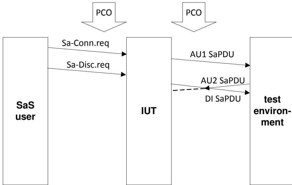
Figure 9 – Revocation during safe connection establishment
