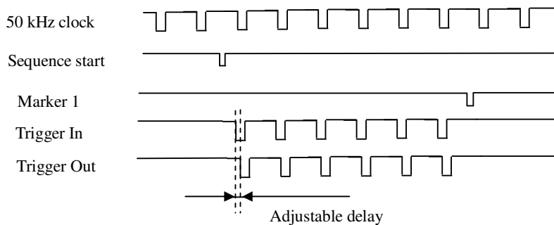
Figure 5: Triggering Timing Diagram
