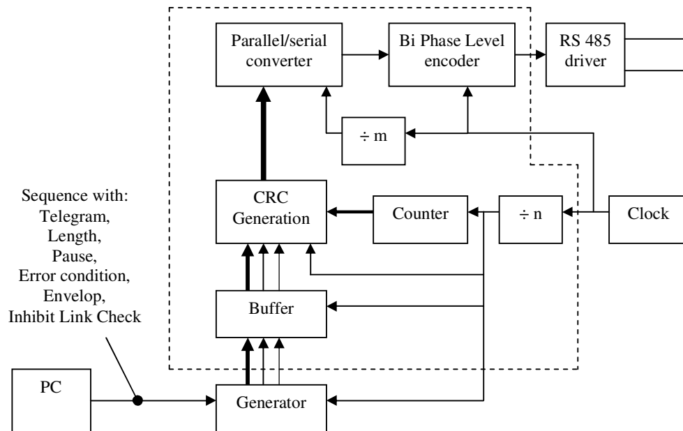
Figure 26: Block Diagram for Interface 'K' Adapter
