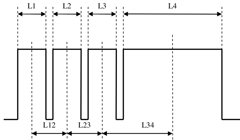
Figure 19: Shape of multiple side lobes, Alternative 2
