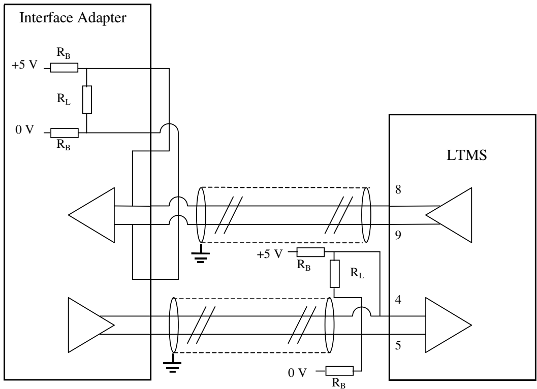
Figure 21: Physical Configuration for Interface ‘Vκ’
