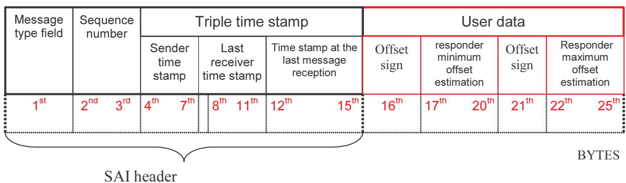
Figure 15: OffsetEst message
