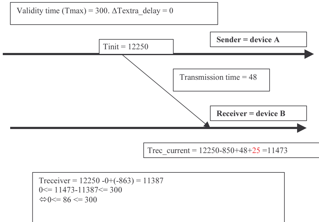
Figure 27: Example of Time stamp procedure and check
