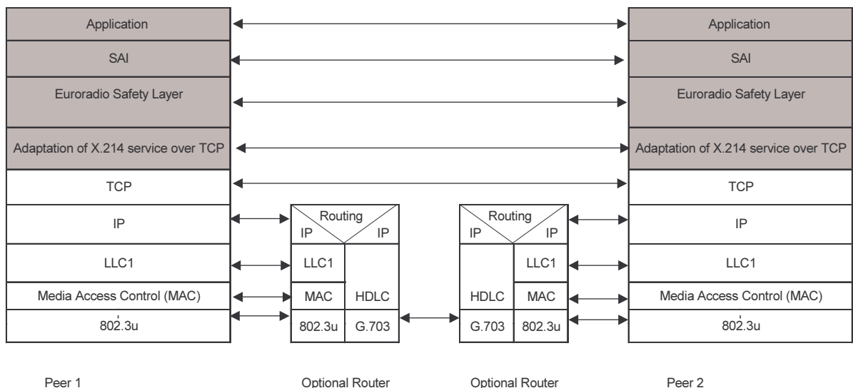
Figure 28: Protocol stacks used to connect an ERTMS application to its counterpart
