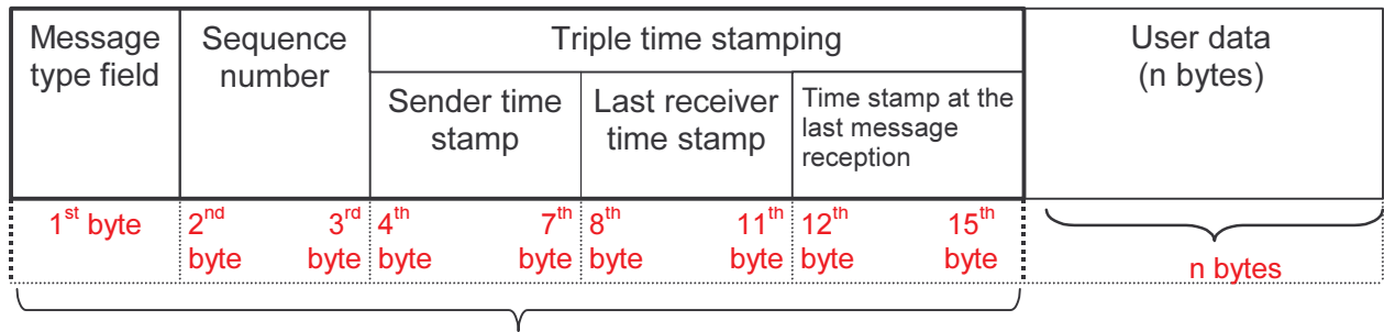
SAI header in case of application data transmission
