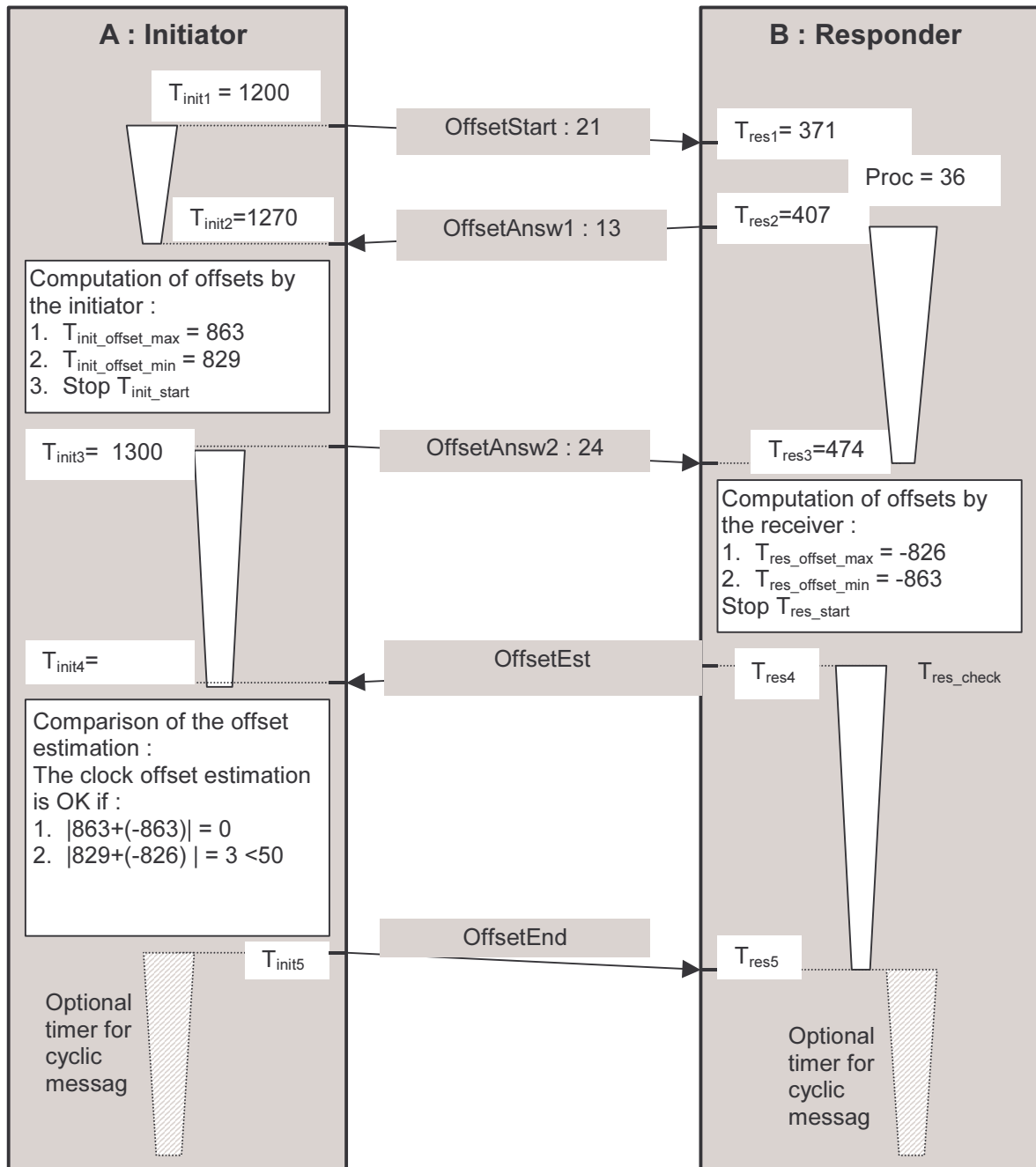
Figure 26: Example of Clock offset update procedure
