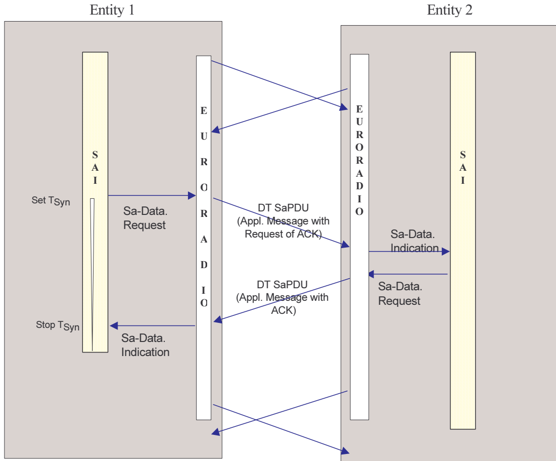
Figure 25: Procedure for detection of network delay
