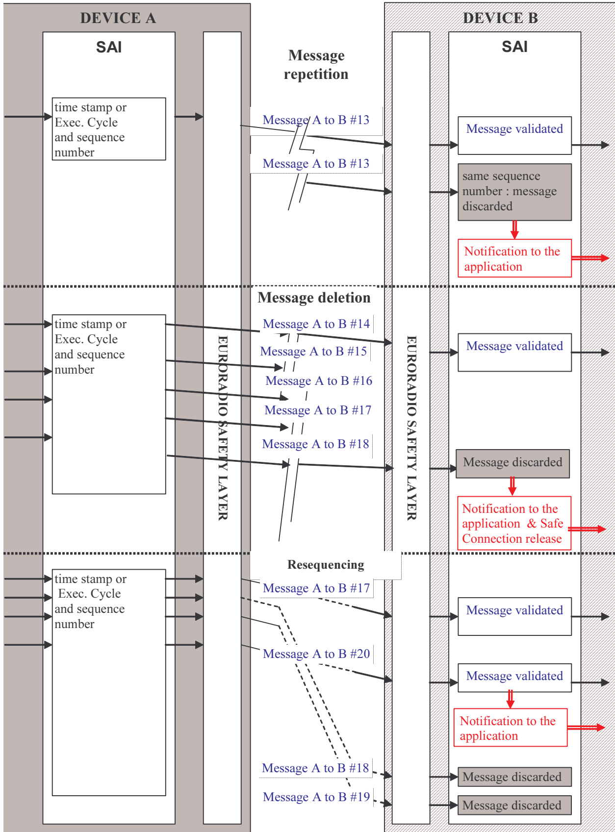
Figure 11: Sequencing errors
