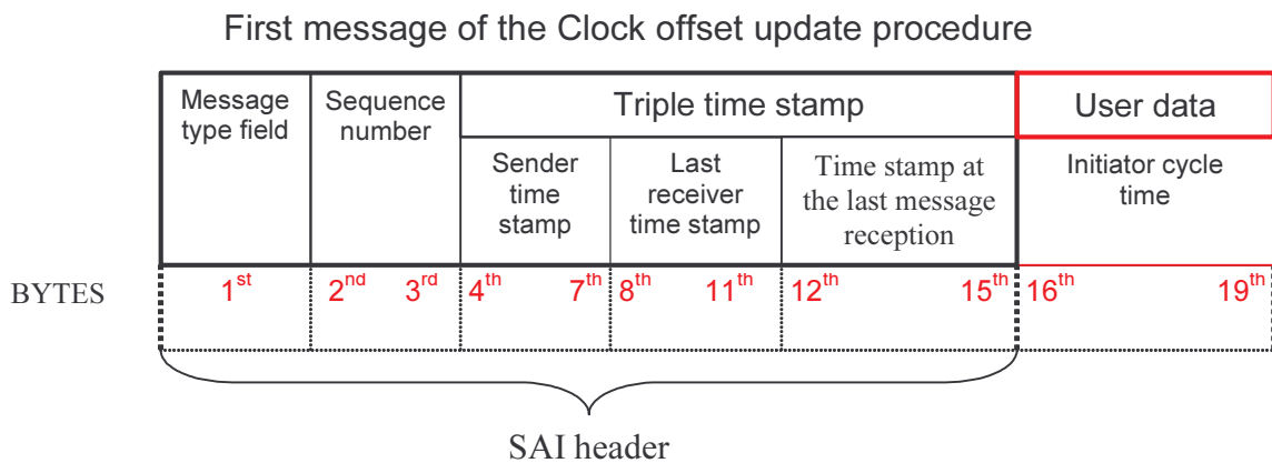
Figure 12: OffsetStart message
