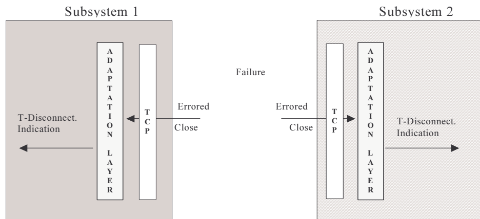
Figure 35: Disruptive Connection release detailed protocol sequence
