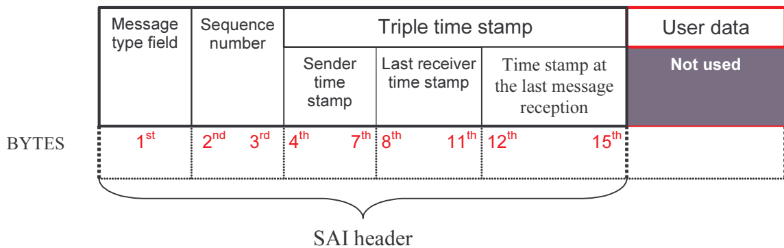
Figure 14: OffsetAnsw2 message
