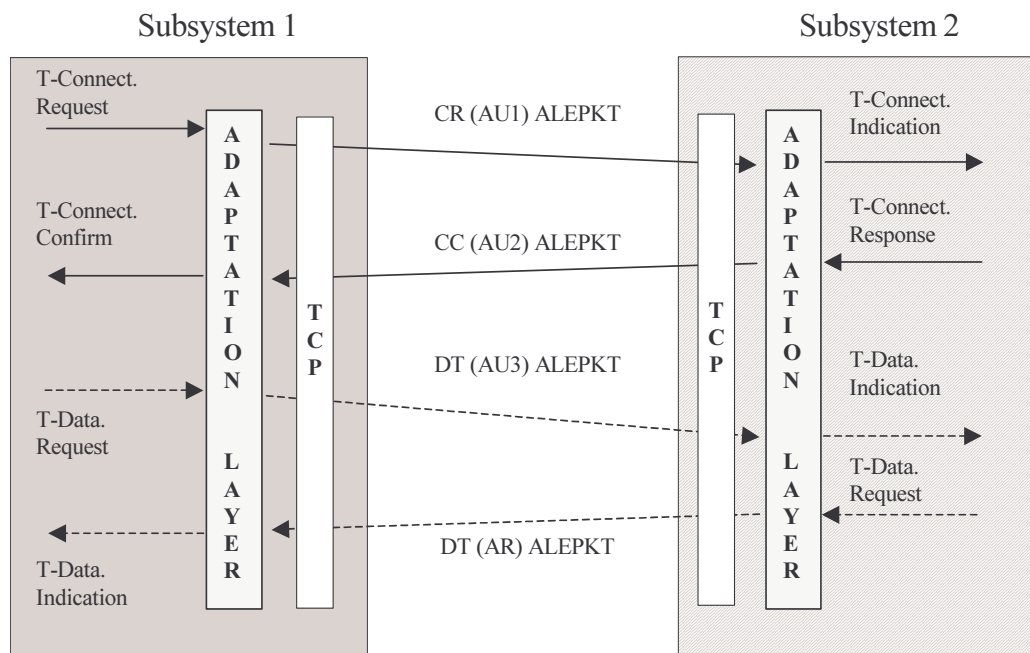
Figure 32: Safe Connection establishment: Detailed protocol sequence
