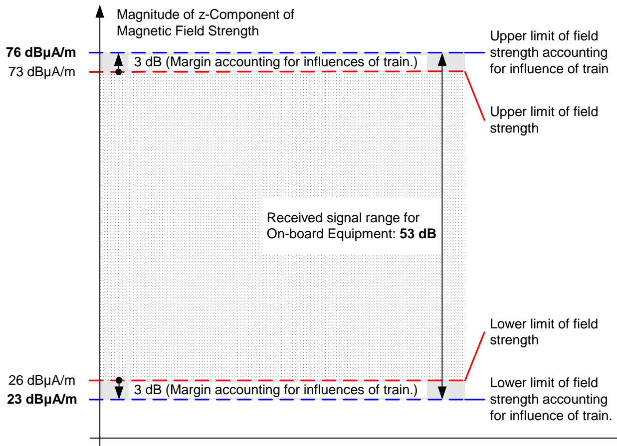
Figure 7-3: Limits of the Magnitude of the z-Component |H_z| of the Magnetic Field Strength H with Margins for On-board Equipment
