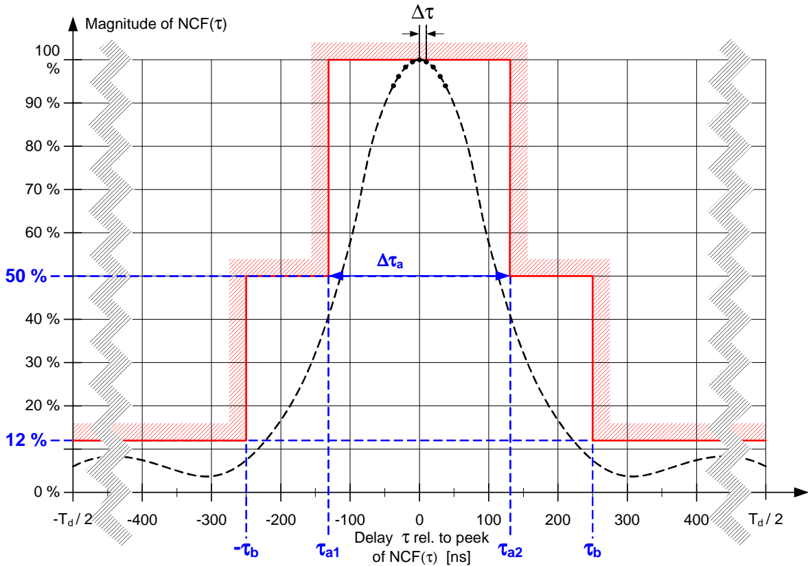
Figure 6-16: Mask for the Normalised Correlation Function NCF(\tau)
