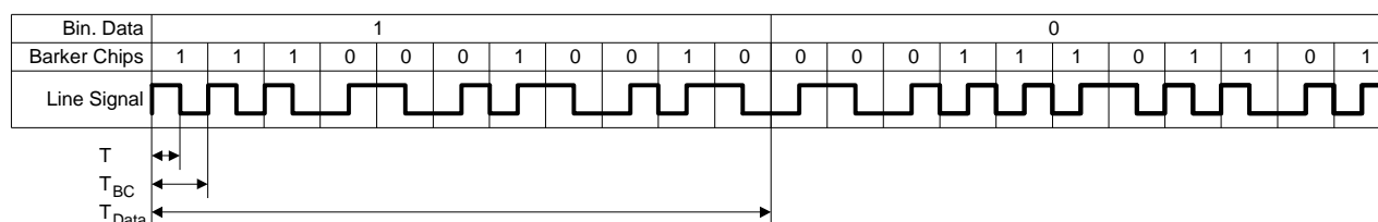
Figure 6-6: Differential Bi-Phase-Level Coding Scheme
