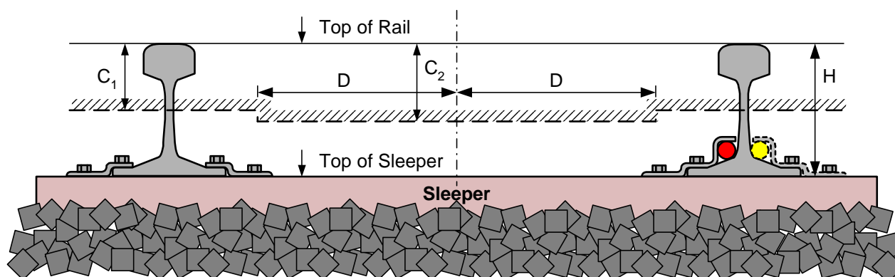
Figure 6-21: Nominal Installation Position of ELC with Indication of Possible Attachment Method to the inner and outer Foot of the Rail
