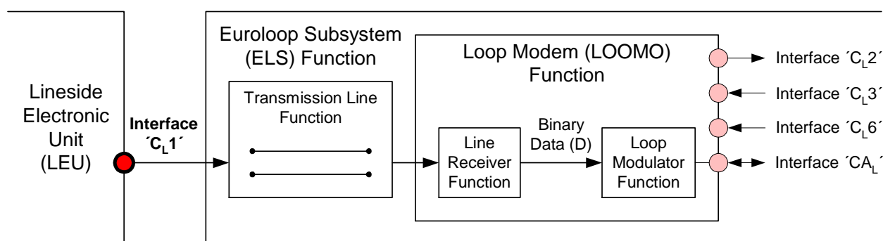
Figure 6-5: Data Transmission between LEU and LOOMO
