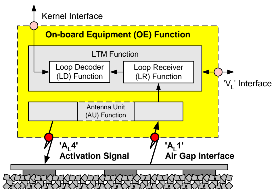
Figure 7-2: Air Gap Interfaces of On-board Equipment
