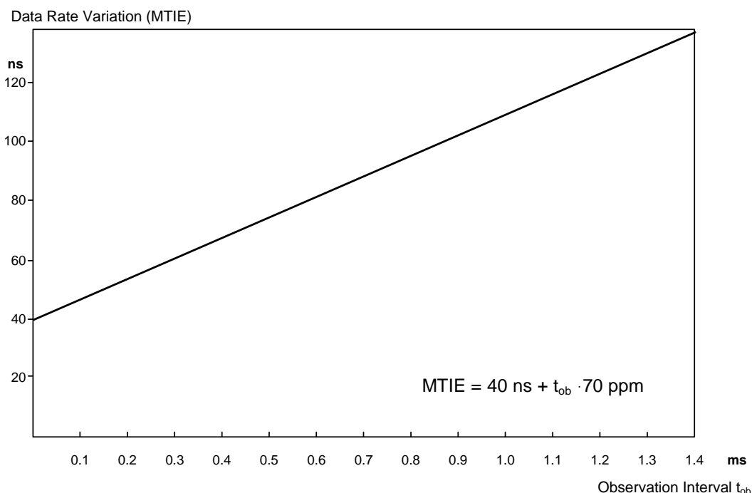
Figure 6-14: MTIE of the Modulation Signal
