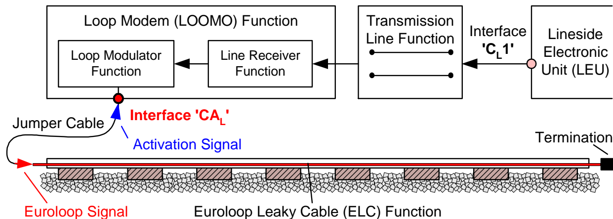
Figure 6-11: Signal Transmission between LOOMO and ELC
