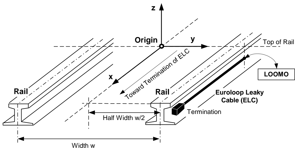
Figure 5-3: Coordinate System
