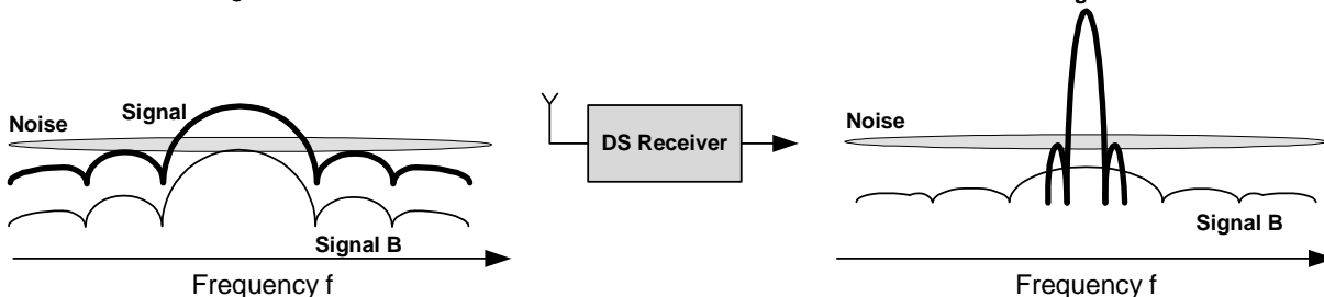
Figure B- 3: Spectral Behaviour of CDMA Signals
