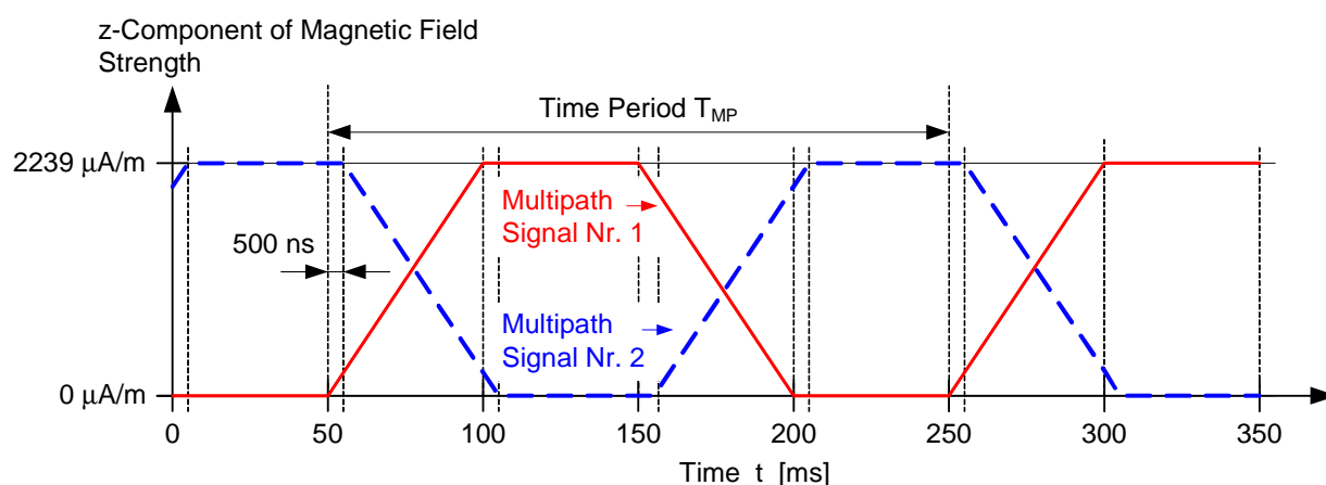
Figure 7-6: Time-Varying Multipath Signals
