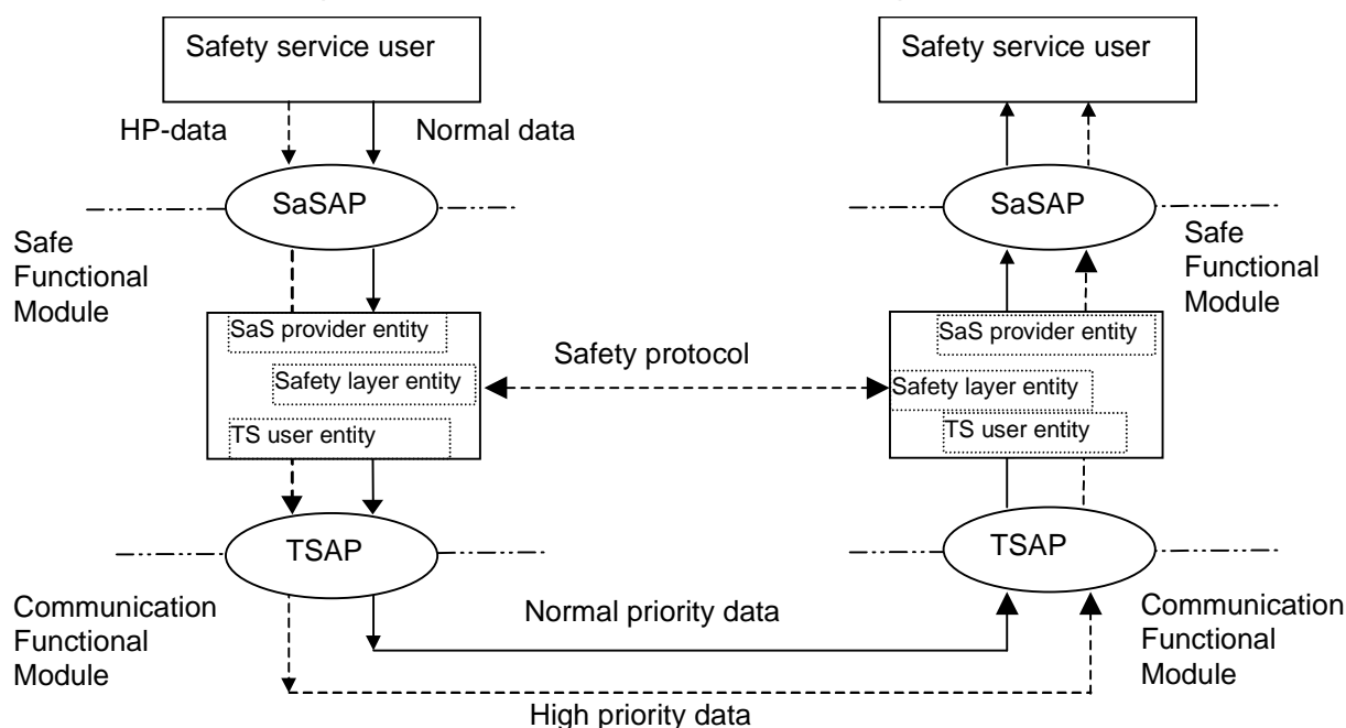
Figure 7 Model of the safe services
