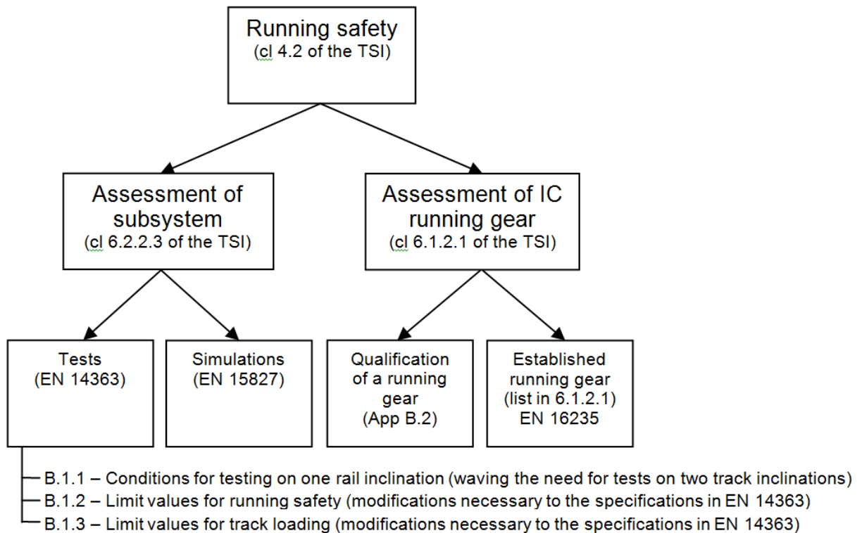
Figure 5: Flow chart of all the possibilities to prove the running safety in the TSI
