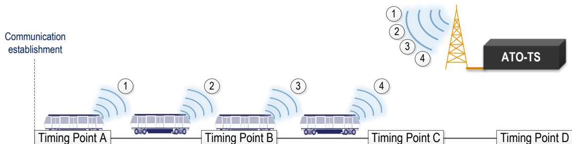
Figure 11 Communication sequence
