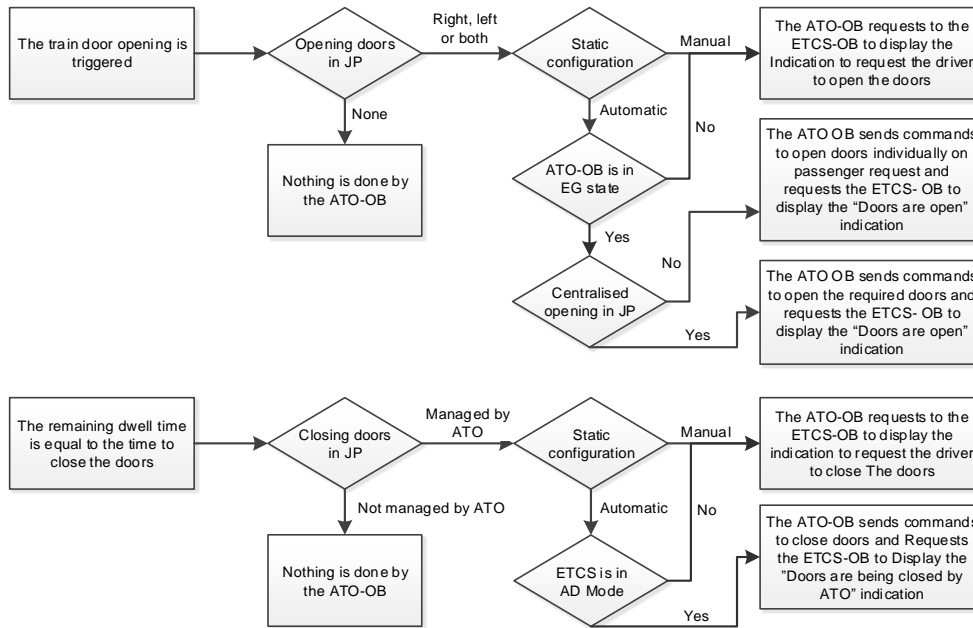
Figure 3 Door operation diagrams
